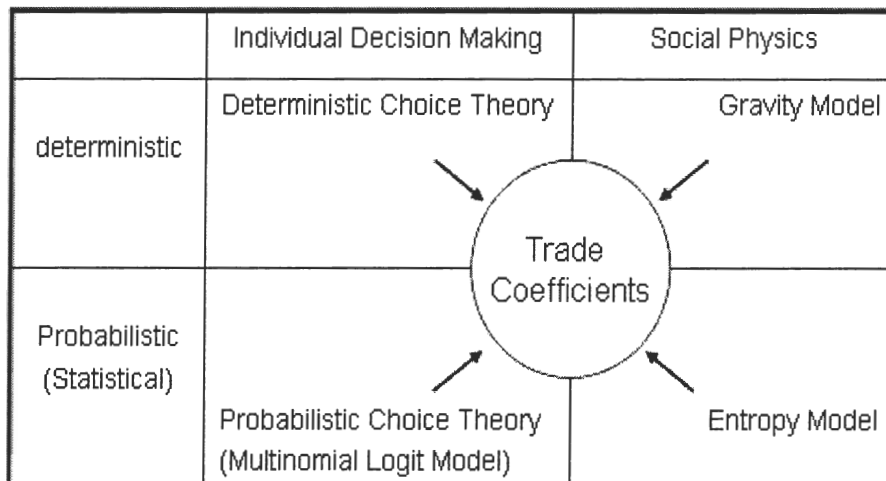
Figure 1: classification
